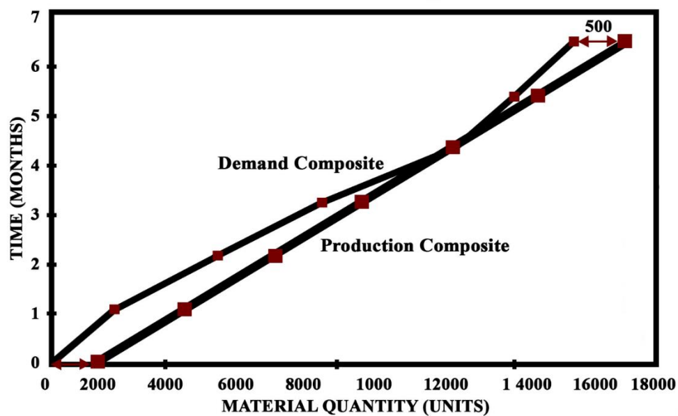
Fig. 2. Composite demand and production in the material (units) - time diagram.
